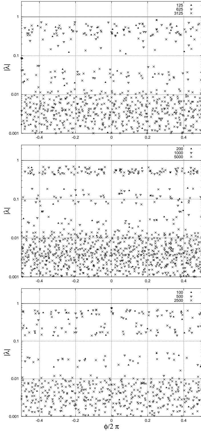
FIGURE 4. Even-parity spectra of the quantum baker's maps B_{5,N} , along geometric sequences N = N_o \times 5^k . The eigenvalues are represented on a logarithmic scale ( \arg \lambda / 2\pi against \log |\lambda| ). The dimensions indicated correspond to N/5 .
