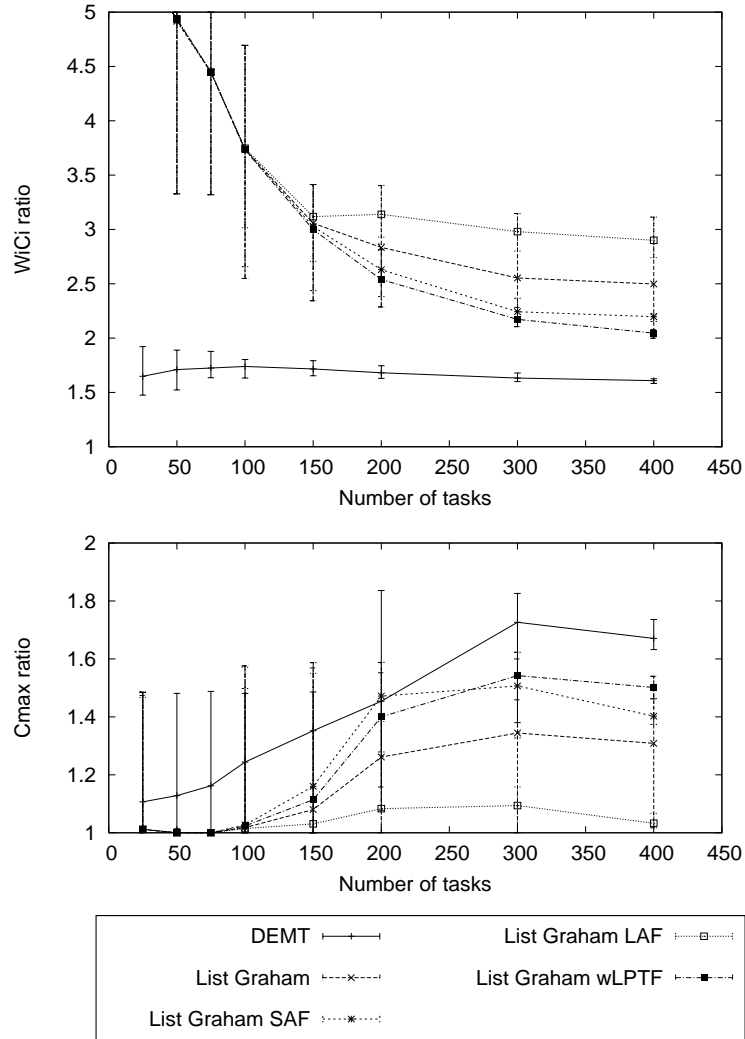
Figure 3: Performance ratio for the simulation on 200 processors, parallel tasks following the Cirne model
