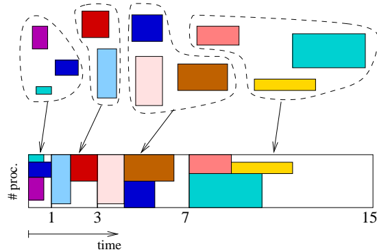
Figure 2: Principle of the bi-criteria algorithm using batches of doubling sizes.
