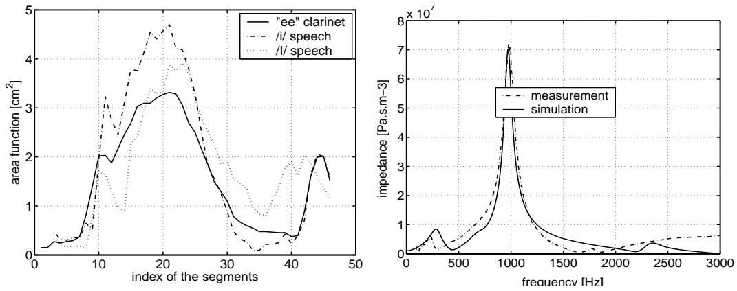
Figure 10: At left: area function for the vowels /i/ and /ɪ/ (data from Story and Titze with glottis added). Also shown are the calculated tract configuration named “ee” by clarinetists, as determined from inversion. The abscissa is the element number: the first two are the glottis (see 4.4), the next 44, of length 4 mm comprise a tract 174 mm long. At right: the impedance spectrum for the “ee” tract configuration measured on one of the authors (player G) an amateur clarinetist.
