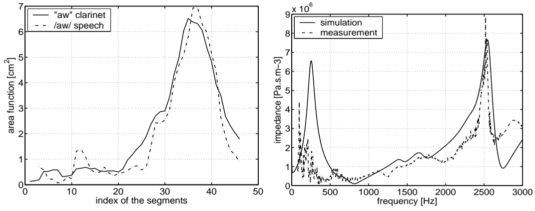
Figure 11: At left: area function for the vowel /a/ (data from Story and Titze with glottis added). Also shown are the calculated tract configuration named “aw” by clarinetists, as determined from inversion. The abscissa is the element number: the first two are the glottis (see 4.4), the next 44, of length 4 mm comprise a tract 174 mm long. At right: the impedance spectrum for the “aw” tract configuration measured on player B.
