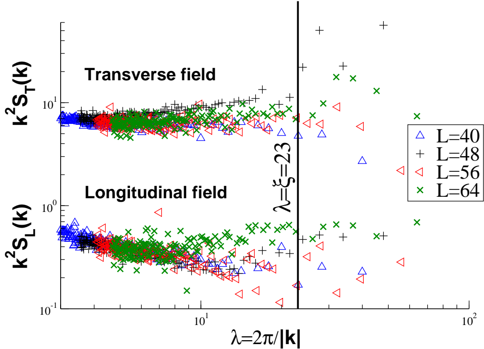
FIG. 7: The squared amplitudes of the Fourier transforms k^2 S_L and k^2 S_T for the div (lower data) and curl (upper data) of the non-affine deformation field (see Eq. (7)) plotted as functions of the wave length \lambda = 2\pi/|\underline{k}| . Different system sizes, as indicated in the figure, have been included to demonstrate that S_L and S_T are essentially system size independent for small \lambda . Note that the statistics deteriorates for large \lambda .
