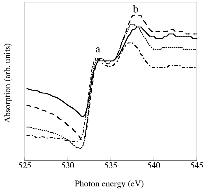
Fig. 5 : Absorption spectra in the vicinity of the O-K edge in the HfO 2 /SiO 2 /Si system calculated from the experimental reflection spectra by means of the Kramers-Kronig relations, for various glancing angles : 2° (solid line), 3° (dashed line), 4° (dotted line) and 5° (dashed-dotted line).
