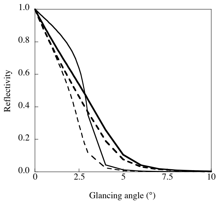
Fig. 3: Reflection coefficients calculated in the framework of the Fresnel approach for HfO 2 (thick line) and SiO 2 (thin line), at 520 eV (solid line) and at 540 eV (dashed line).
