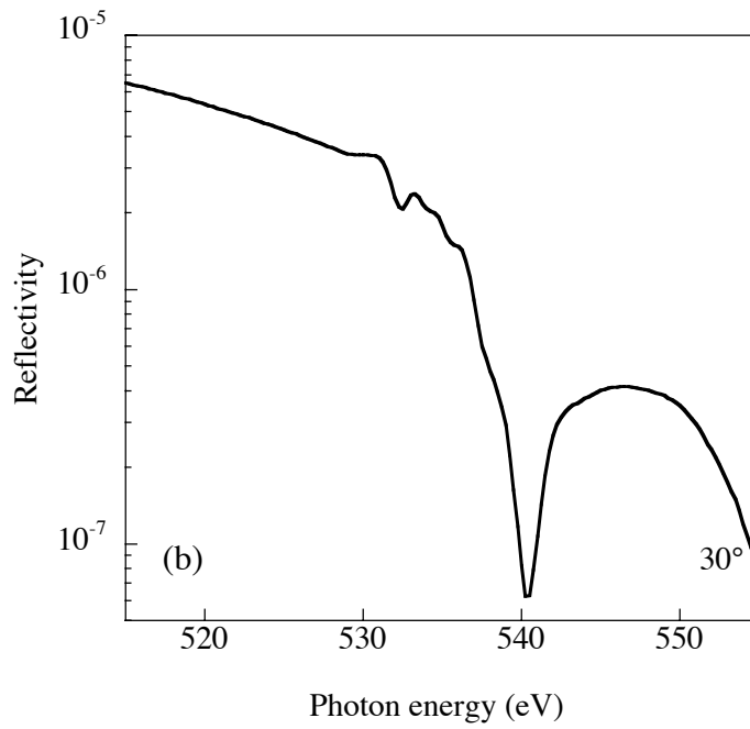
Fig. 1: Reflection spectra of the \text{HfO}_2/\text{SiO}_2/\text{Si} system for various glancing angles between 2 and 10^\circ (a) and for 30^\circ (b).
