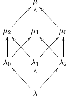
FIGURE 4. A commutative diagram of semilattice-valued distances.
