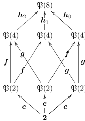
FIGURE 3. The cube \mathcal{D}_{\text{ac}} , unliftable by V-distances of type 3/2.
