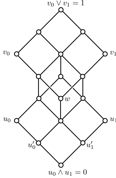
FIGURE 2. The distributive lattice D .
