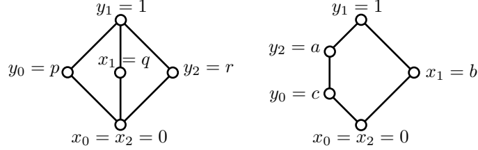
FIGURE 1. The decorations of M_3 and N_5 .
