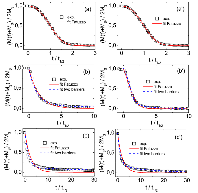
Fig. 3. Relaxation measurements (symbols) measured for samples I (top), II (middle) and III (bottom) for the descending (a,b,c) and ascending (a',b',c') branches of the hysteresis loops. Full lines represent the fits using Fatuzzo's model (2). The dotted lines are the fits considering the presence of two energy barriers.
