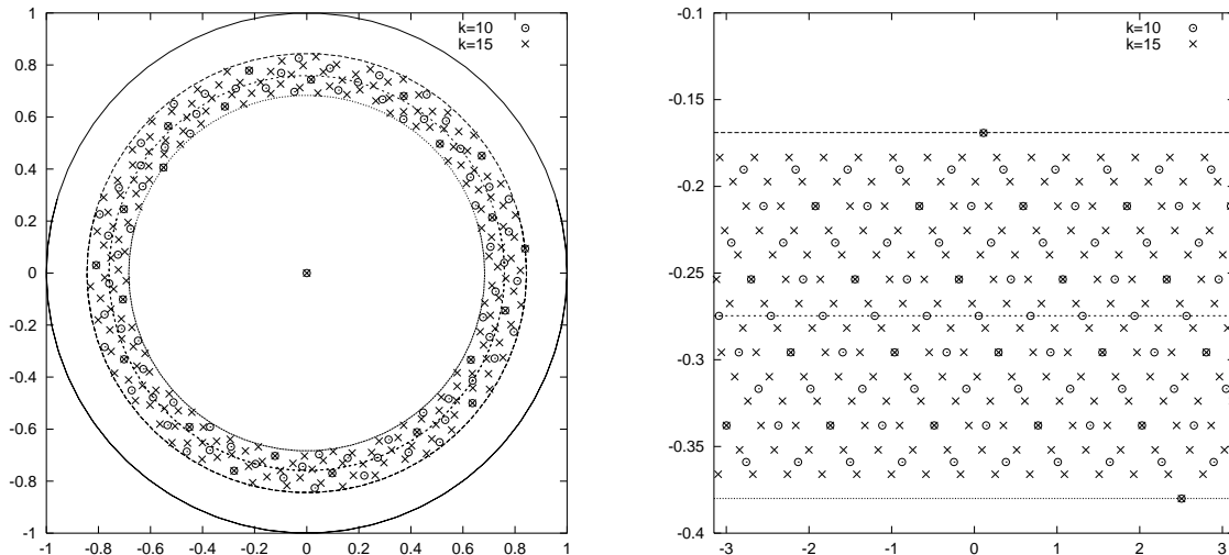
FIGURE 1. The illustration of Theorem 1: on the left, eigenvalues \lambda \in \text{Spec}(\tilde{B}_h) for (2\pi h)^{-1} = N = 3^{10} (circles) and for N = 3^{15} (crosses). The four circles correspond to radii 1, |\lambda_+| , |\lambda_+\lambda_-|^{\frac{1}{2}} , |\lambda_-| , where \lambda_{\pm} are given in Proposition 6.5. The critical radius in the statement of the theorem is here r_0(\tilde{B}) = |\lambda_+\lambda_-|^{\frac{1}{2}} (dotted line). On the right, we plot the phase (horizontal) and modulus (vertical, log scale) of these eigenvalues. The eigenvalues appear with high, varying, multiplicities which peak on the circle |\lambda| = r_0(\tilde{B}) , but the angular distribution is asymptotically uniform.
