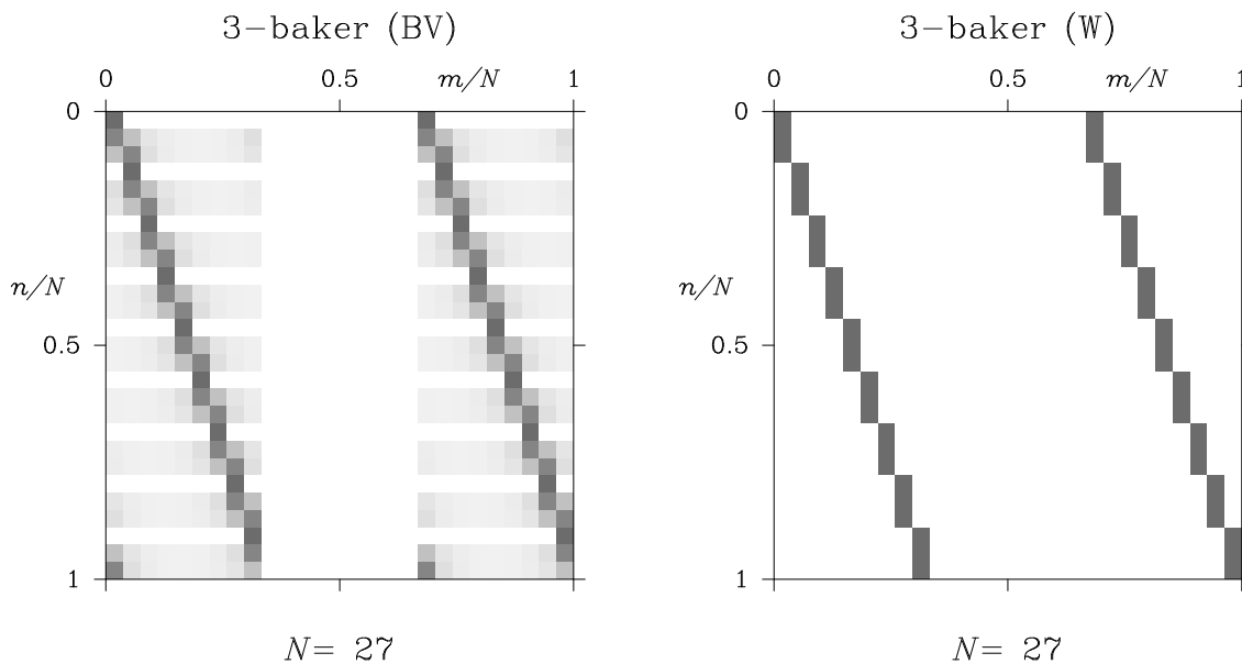
FIGURE 9. Matrices B_{27} (left) and its toy model \tilde{B}_{27} (right) for the quantum 3-baker. The gray scale corresponds to the moduli of the matrix elements, (white = 0, black = 1).
