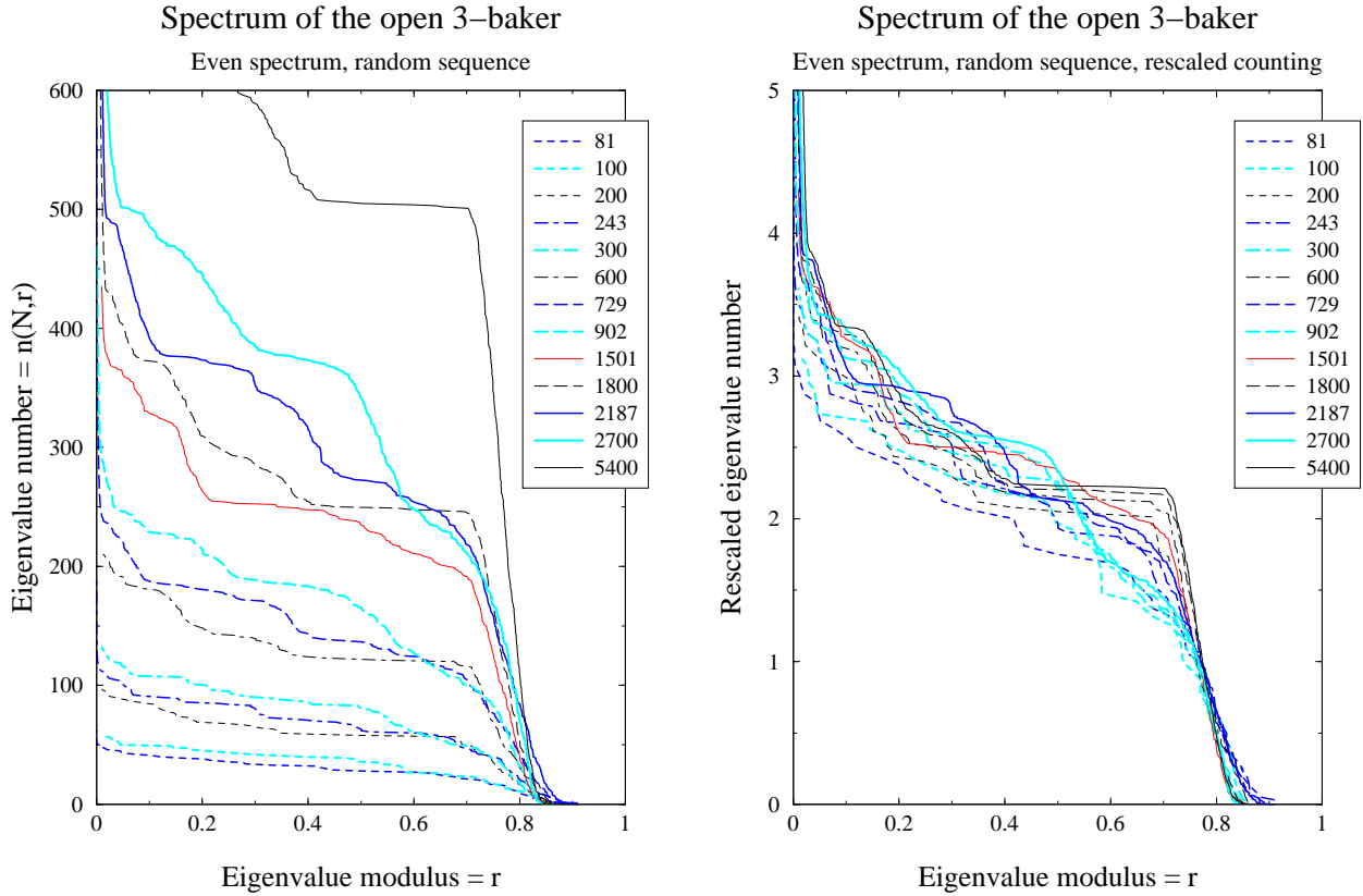
FIGURE 7. On the left, we plot the number n(N, r) of even eigenvalues of modulus \geq r of the 3-baker B_h (the numbers in the box are the ranks N/3 of the desymmetrized matrices). On the right we have rescaled that number by the factor N^{-\log 2/\log 3} . Data belonging to the same geometric sequence share the same color (online) or linewidth.
