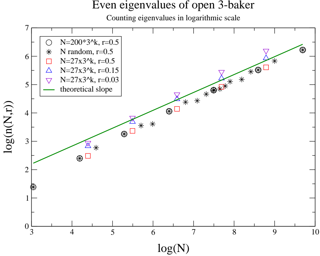
FIGURE 8. Checking the N -dependence of n(N,r) for various values of r , along geometric and arbitrary (*) sequences for N (colors online).
