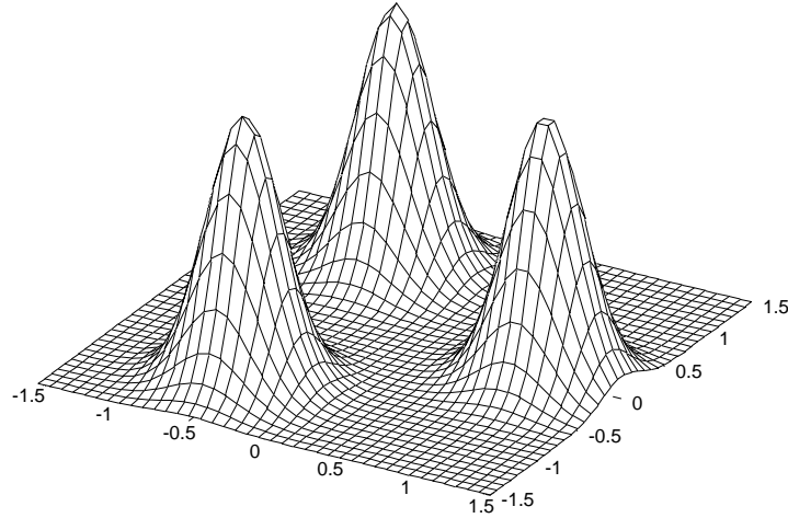
FIGURE 2. A three bump potential exhibiting hyperbolic dynamics in a range of energies.
