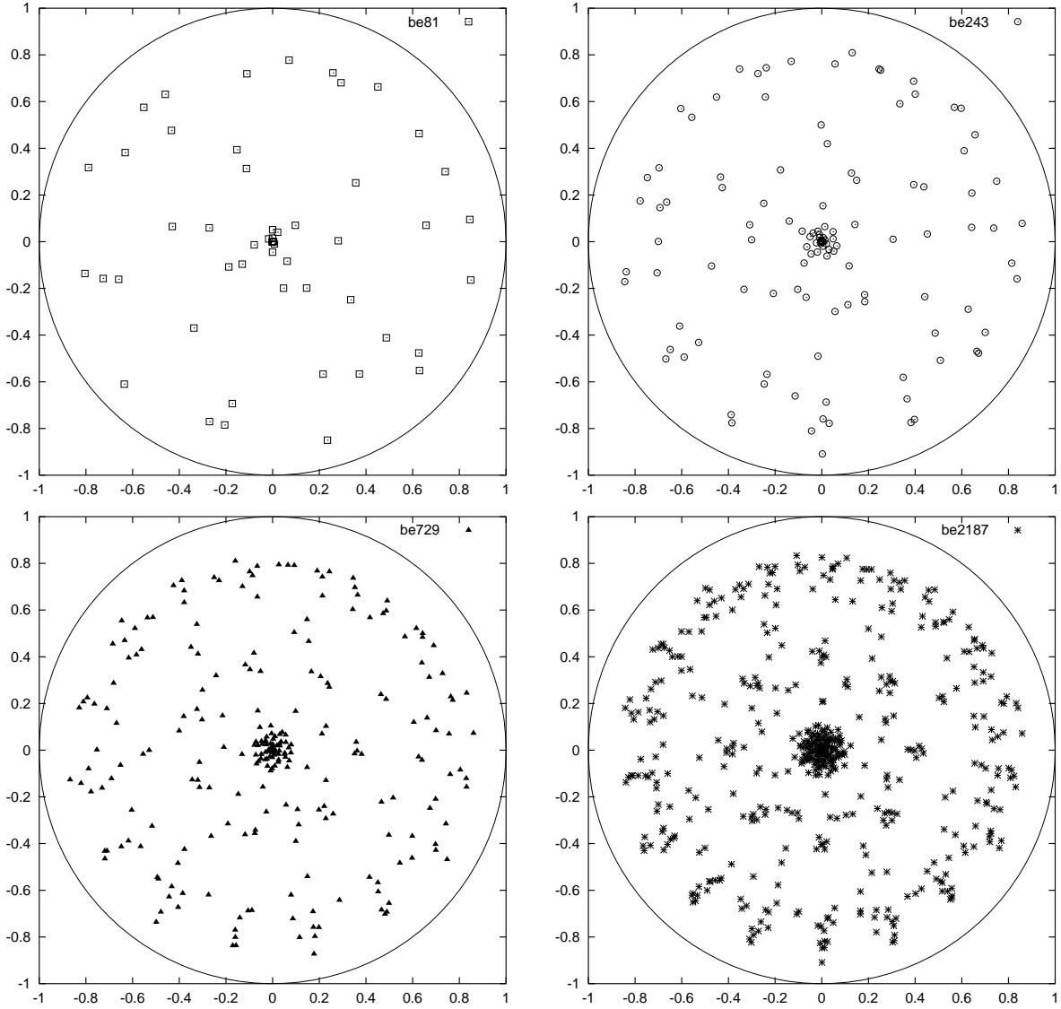
FIGURE 6. Even spectrum of the quantum 3-baker's relation B_h for N/3 = 81, 243, 729, 2187 .
