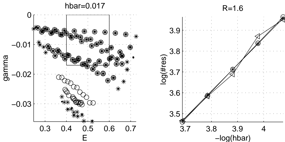
FIGURE 4. A sample of results of [30]: the plot on the left shows resonances for the potential of Fig. 2 ( h = 0.017 ). On the right is the log-log plot of the number of resonances vs. h ; \triangleleft denote numerical data, * the density predicted by the fractal Weyl law, and \circ the least square interpolants.
