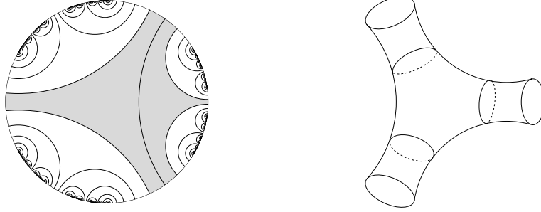
FIGURE 3. An example of \mathbb{H}^2/\Gamma where \Gamma is generated by compositions of reflections in three discs.
