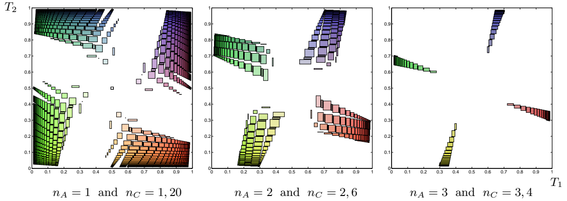
Figure 15: Colour plots of (n_A, 1, n_C, \rho) -regular orbit existence domains in the threshold plane for a = 0.842 . See text for details.
