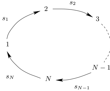
Figure 1: A feedback circuit of N genes.
