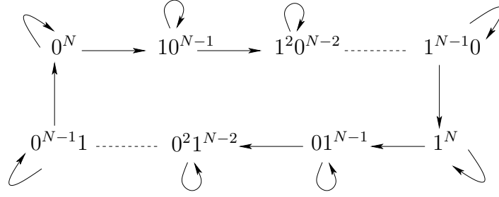
Figure 16: Part of the symbolic graph associated with the negative N -circuit. The nodes represent the symbol vectors \{\theta_i\}_{i=1,N} .
