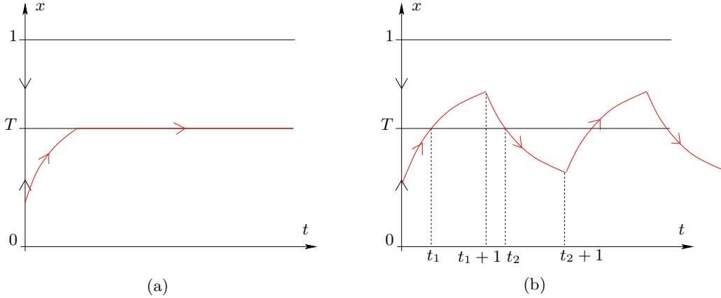
Figure 6: Trajectories in the continuous time self-inhibitor without delay (a) and with delay \tau = 1 (b).
