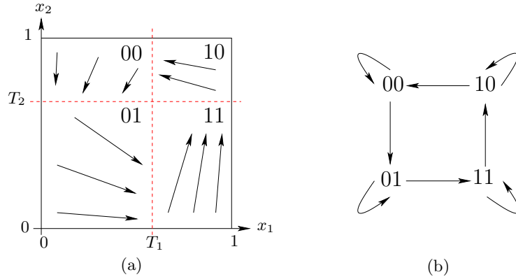
Figure 9: The negative 2-circuit. (a) Atoms in phase space with affine dynamics and directions of motions. (b) Associated symbolic graph.
