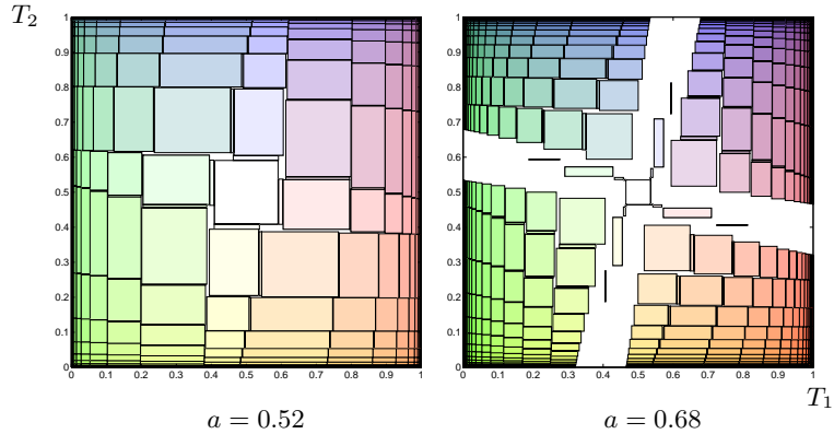
Figure 14: Colour plots of the existence domains in the threshold plane (T_1, T_2) of some regular orbits for a = 0.52 and a = 0.68 . The orbits are characterised by one iteration per winding in any two consecutive atoms, p iteration(s) per winding in a third atom and \rho iteration(s) per winding in the remaining atom. On each picture, the domains where all orbits pass one iteration in 10 and in 00 – the (p, \rho) -regular orbit – concern the right upper quadrant (red and blue). Light (resp. dark) red corresponds to small (resp. large) p , i.e. number of iteration(s) per winding in 01. Light (resp. dark) blue corresponds to small (resp. large) \rho , i.e. (mean) number of iteration(s) per winding in 11. The domains where the orbits pass one iteration in 00 and in 01 concern the left up quadrant, etc. See text for further details.
