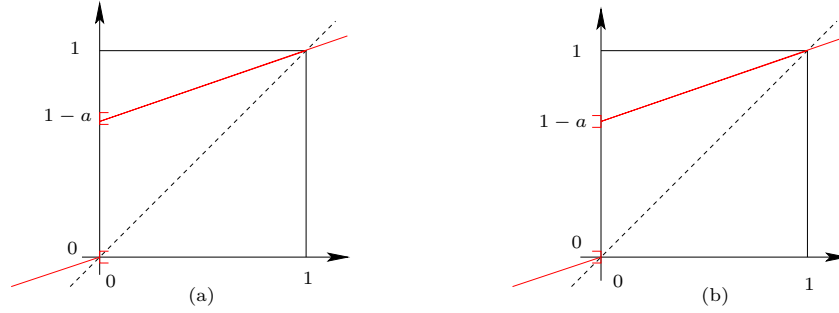
Figure 3: (a) Graph of the map F(x) = ax + (1 - a)H(x) . The point 0 is a ghost fixed point. It attracts all initial conditions x < 0 but is not a fixed point. The point 1, obtained from 0 by applying the symmetry S is a true fixed point. (b) Assuming H(0) = 0 instead of H(0) = 1 in the definition of F changes the ghost fixed point to a genuine fixed point.
