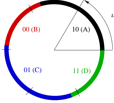
Figure 13: A regular orbit code is generated by a rigid rotation on the unit circle x \mapsto x + \nu \pmod 1 composed by 4 arcs. Each arc (specified by a colour) is associated with an atom of the partition. Here \nu = \frac{1}{6} and the generated code is (10^2 00 01^2 11)^\infty and is 6-periodic.
