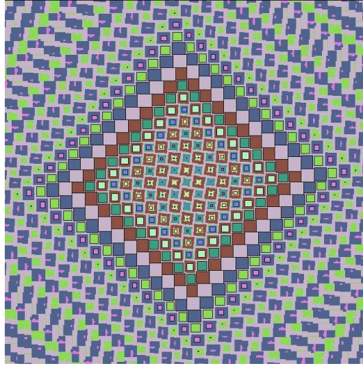
Figure 11: Colour plot of basins of attractions in the square [0.425, 0.575]^2 for the negative 2-circuit for a = 0.99 and T_1 = T_2 = \frac{1}{2} – obtained from a numerical simulation. The picture shows that there are only balanced orbits. Several immediate basins – characterised by products of intervals – clearly appear. For instance, sea-green squares correspond to the balanced orbit with p = 8 , brown squares to the orbit with p = 9 , thistle squares to the orbit with p = 10 , etc. In the present case, the balanced 4p -periodic orbits are known to exist for p = 1, \dots, 14 (indeed we have a_{14} < 0.99 ).
