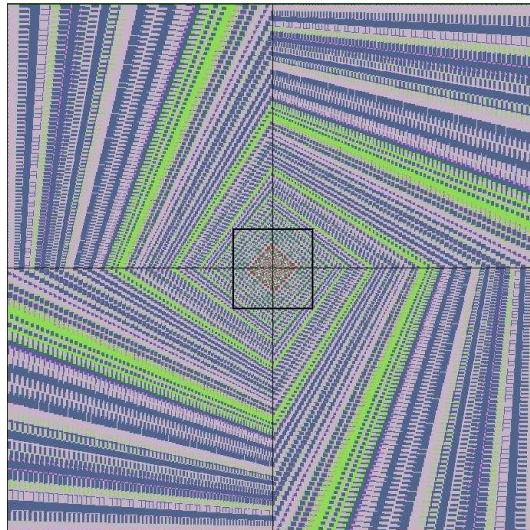
Figure 12: Colour plot of the basins of attraction in the square [0, 1]^2 (complete phase space) for the negative 2-circuit with parameters as in Figure 11 (i.e. a = 0.99 and T_1 = T_2 = \frac{1}{2} ). The picture clearly shows that any orbit has a spiral trajectory toward some balanced orbit located in the region – delimited by the square – displayed in Figure 11.
