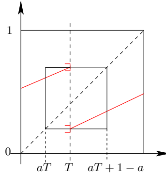
Figure 4: Graph of the map F(x) = ax + (1-a)H(T-x) together with the invariant absorbing interval [aT, aT + 1 - a] .
