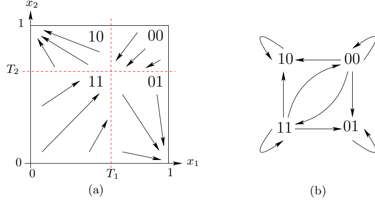
Figure 7: The positive 2-circuit. (a) Atoms in phase space with affine dynamics and directions of motions. (b) Associated symbolic graph.
