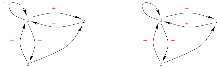
Figure 2: A network with 3 nodes and the corresponding network obtained by flipping the signs of incoming and outgoing arrows from the node 1, excepted the self-interaction sign.
