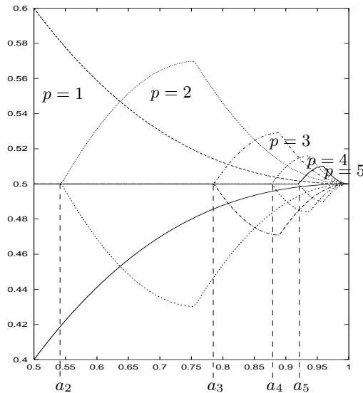
Figure 10: The negative 2-circuit. Projections of parameter domains of existence of balanced orbits – for p = 1, 5 – on the plane (a, T_1) (or by symmetry on the plane (a, T_2) ). The representation here differs from Figure 8 (intersections with planes a = \text{constant} in threshold space). A representation as in Figure 8 would have presented nested squares centred at (\frac{1}{2}, \frac{1}{2}) and symmetric with respect to the diagonal; the number and the size of squares depending on a .
