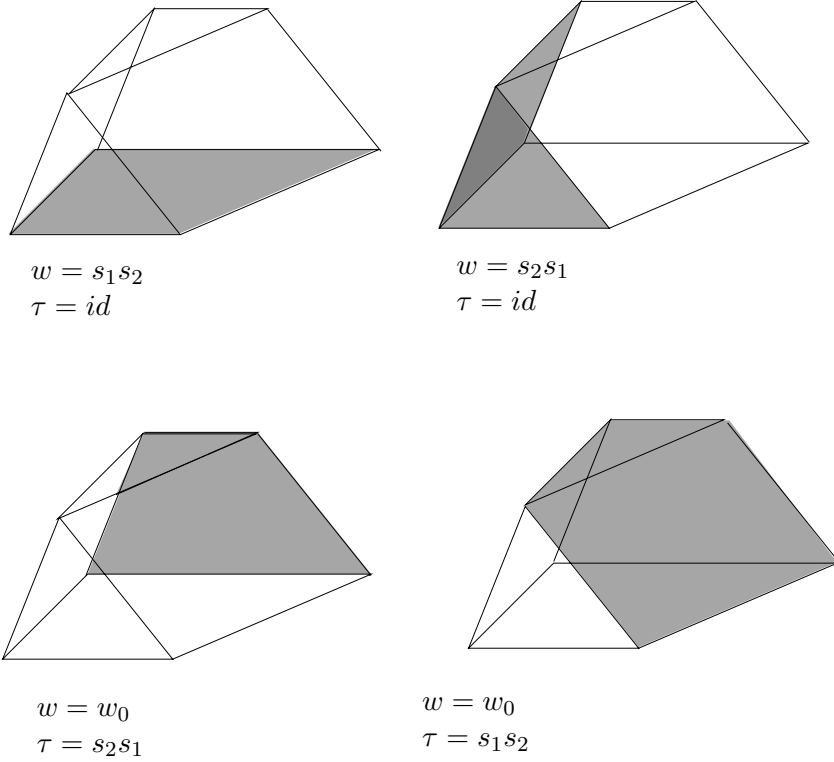
FIGURE 3.4. Faces \mathcal{C}_1^{w,\tau}(\lambda_0) in the polytope \mathcal{C}_i(\lambda_0)
