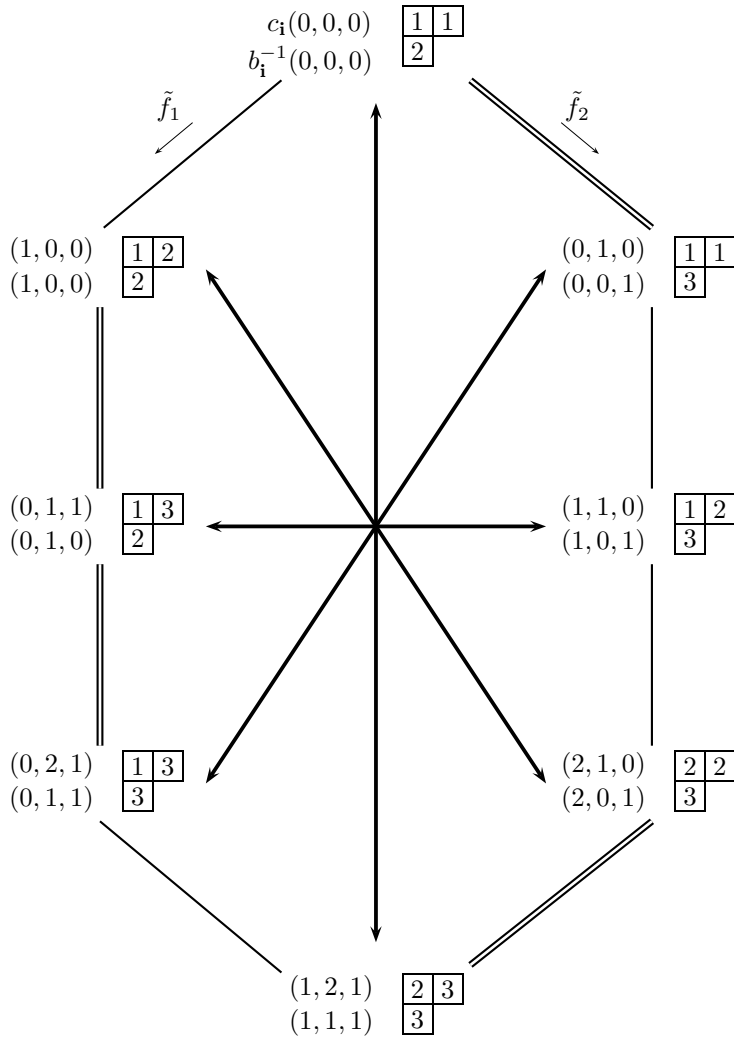
FIGURE 2.2. Schützenberger involution in \mathcal{B}(\varpi_1 + \varpi_2) .
