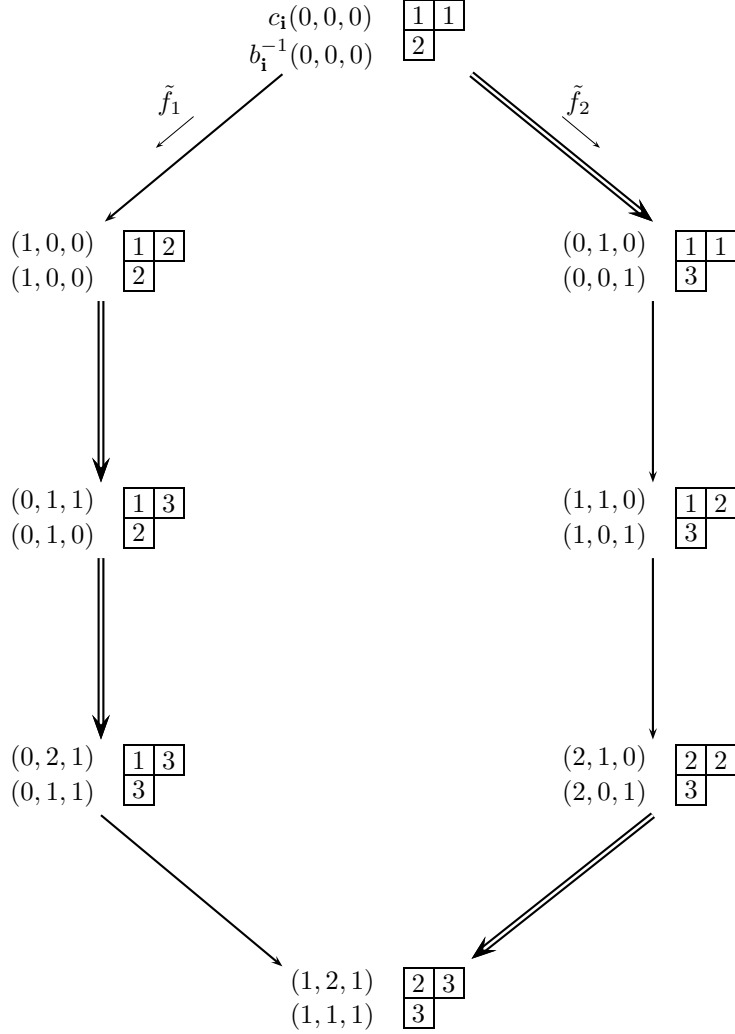
FIGURE 1.1. Parametrizations of the basis \mathcal{B}(\varpi_1 + \varpi_2)
