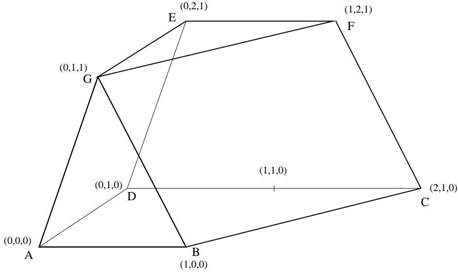
FIGURE 3.3. Polytope \mathcal{C}_{\mathbf{i}}(\mathcal{B}(\varpi_1 + \varpi_2))
