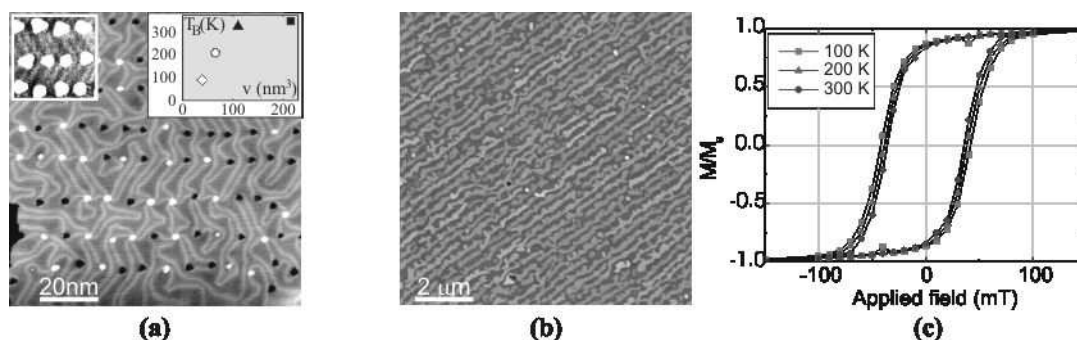
Figure 4. (a) STM image of a SO Co/Au(111) system during the fabrication of pillars. Inset: Conventional SO Co/Au(111) dots in the sub-AL range (left) and blocking temperature of pillars as a function of their volume [50] (right) (b) SO Fe/W/Mo(110) stripes, 4.3 nm-thick [95] (c) magnetization loops of Fe/W(110), 5.5 nm-thick, along in-plane [001].
