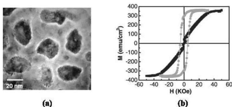
Figure 5. SO ferrimagnetic CoFe 2 O 4 columns in a BaTiO 3 ferroelectric matrix. (a) plane view (b) magnetization loops performed at 300 K for perpendicular (shaded) and in-plane (dark) field [9].
