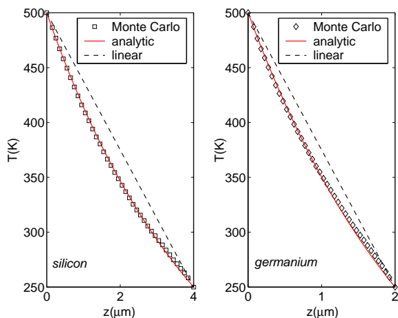
FIG. 8: Steady state temperature in Fourier's regime for silicon and germanium in the case of a large thermal gradient; comparison to the heat conduction equation analytical solution for temperature dependent conductivity.
