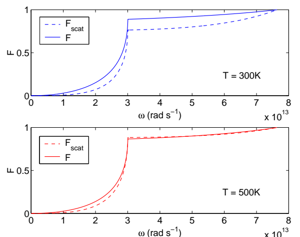
FIG. 3: Normalized number density function in silicon with and without P_{scat} correction
