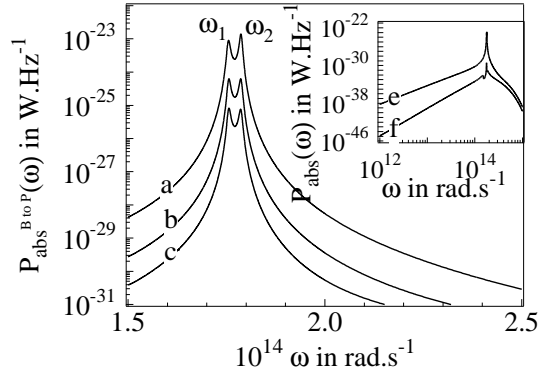
Fig. 20. Mean power radiated by the bulk (at T_B = 300 K) and absorbed by the particle (of radius a=5 nm) versus frequency. (a) d=20 nm; (b) d=50 nm; (c) d=100 nm. The insert (log-log scale) shows the spectrum of the absorbed power between 10^{12} rad s ^{-1} and 10^{15} rad s ^{-1} ; (e) d=20 nm; (f) d=1 mm. From [94]
