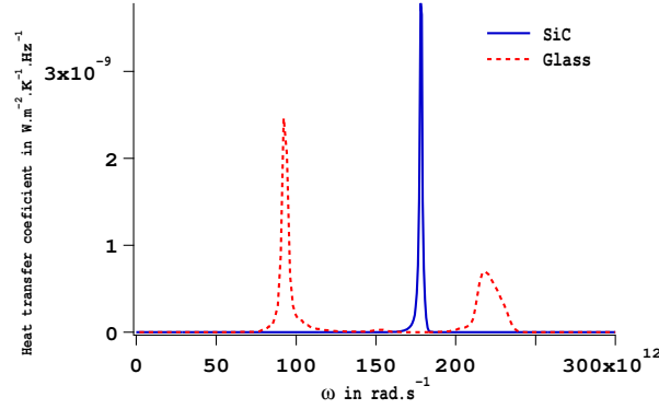
Fig. 18. Monochromatic heat transfer coefficient for a distance d = 10 nm and a temperature T = 300 K. From [85]
