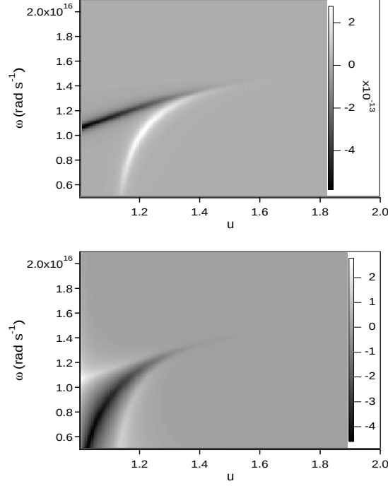
Fig. 26. Same as Fig.25 but for d = 100 nm. From [120]
