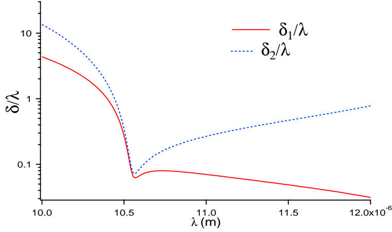
Fig. 4. Surface wave decay length along the z -direction in medium 1 and 2 versus the wavelength for a SiC-vacuum interface.
