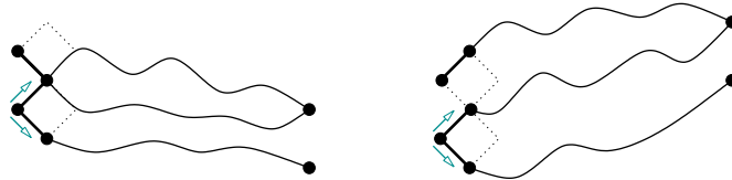
FIGURE 2. The first three steps in an osculating (0, 1) -star.
