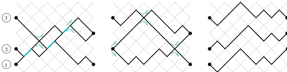
FIGURE 1. A non-crossing configuration, an osculating configuration, and a non-intersecting (vicious) configuration.
