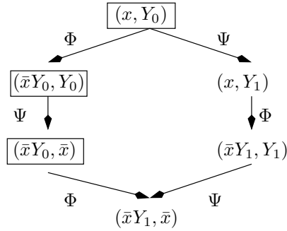
FIGURE 4. The orbit of (x, Y_0) under the action of \Phi and \Psi .
