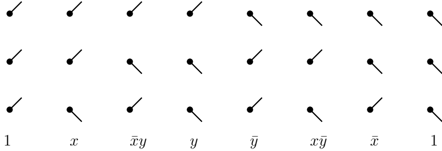
FIGURE 3. The eight possible moves.
