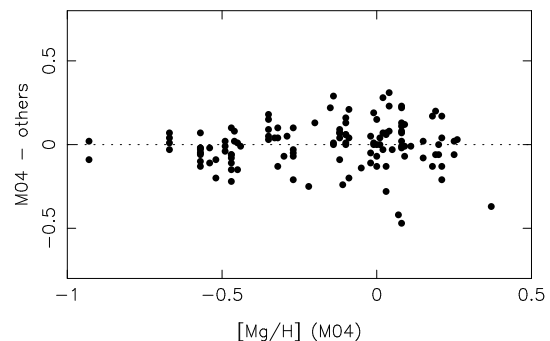
Fig. 1. Comparison of [Mg/H] computed under NLTE approximation by M04 and LTE [Mg/H] computed by the other authors. No systematic trend can be observed. The mean difference is null, the dispersion 0.13 dex for 126 stars in common.
