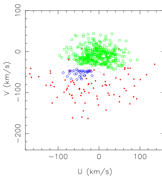
Fig. 8. The sample of 639 stars plotted in the (U,V) plane. Thick disk stars are represented by red dots, thin disk stars by open green squares and Hercules stars by open blue circles. The small dots correspond to stars which could not be classified into the 3 subgroups.
