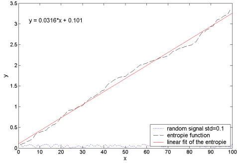
Figure 2. Entropy of y(x) and the smooth function of y(x)=0.0316x+0.101
