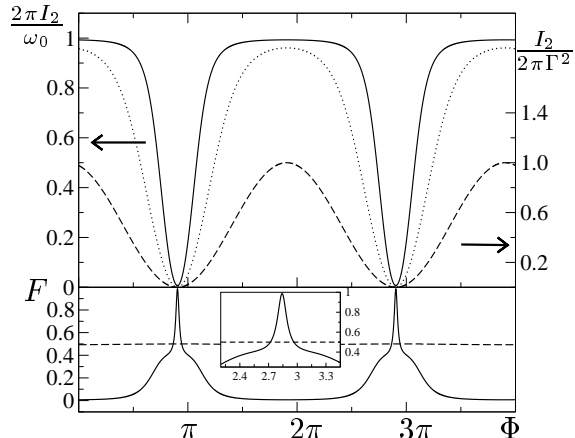
FIG. 2: Upper part: transmitted current I_2 as a function of the AB phase \Phi , for 2 QPCs with \nu = 1/2 and equal tunneling amplitudes \Gamma , with \omega_0\Delta/v_F = 0.3 , and 8\pi\Gamma^2/\omega_0 = 0.01 (dashed curve, right y axis), 1 (dotted curve, left axis), 100 (full curve, left axis). Lower part: Fano factor F = S_2/(2eI_2) as a function of \Phi for the same parameters, 8\pi\Gamma^2/\omega_0 = 100 (full curve), 0.01 (dashed curve, extremely narrow peaks have been removed for the sake of clarity). Inset: zoom on one of the narrow peaks of F for 8\pi\Gamma^2/\omega_0 = 100 .
