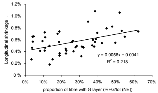
Fig. 9. Relation between longitudinal shrinkage and proportion of fibre with G layer.
