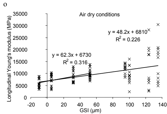
Fig. 8. Relation between Longitudinal Young's modulus and GSI. wet conditions and air dry conditions. x : all GSI ; * : GSI < 60µm.
