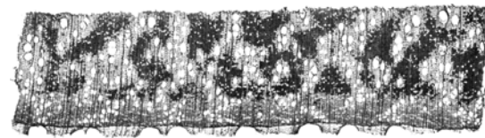
Fig. 4. Azure II staining of chestnut tension wood. Dark zones are fibres with gelatinous layer (scale bar = 500 µm).
