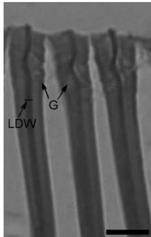
Fig. 3: Longitudinal section of poplar tension wood fibres showing an increase in the G-layer thickness near the cutting surface. LDW = Lignified Double wall ( S_2+S_1+P+intercellular\ layer+P+S_1+S_2 ), G = G-layer. Scale bar = 10 μm.
