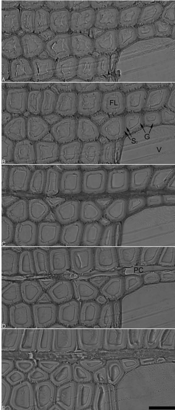
Fig. 1. Transverse sections of poplar tension wood illustrating changes in the shape and thickness of the G-layer in relation to the distance (D) to the cutting surface -- A: D=2 \mu\text{m} -- B: D=14 \mu\text{m} -- C: D=24 \mu\text{m} -- D: D=42 \mu\text{m} -- E: D=150 \mu\text{m} . -- FL=fibre lumen, G=G layer, S 2 =S 2 layer, V=vessel, PC = parenchyma cell. -- Scale bar = 20 \mu\text{m} .
