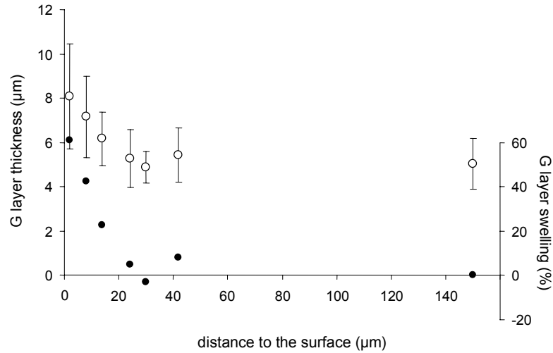
Fig. 2: G-layer mean thickness (empty circle) and standard deviation versus distance to the cutting surface (made after 50 measurements) and the corresponding swelling (full circle) taking measurements at 150 μm as reference.
