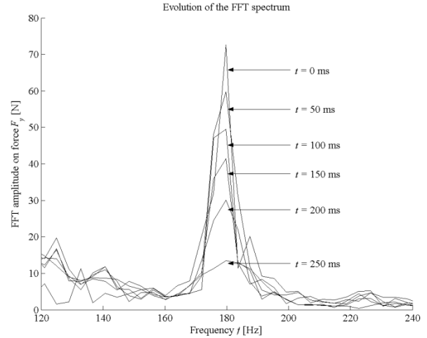
Fig. 10. Spectral density of the dermatome motor as a function of time after a blade jamming at t = 0 ( M = 256 ).
