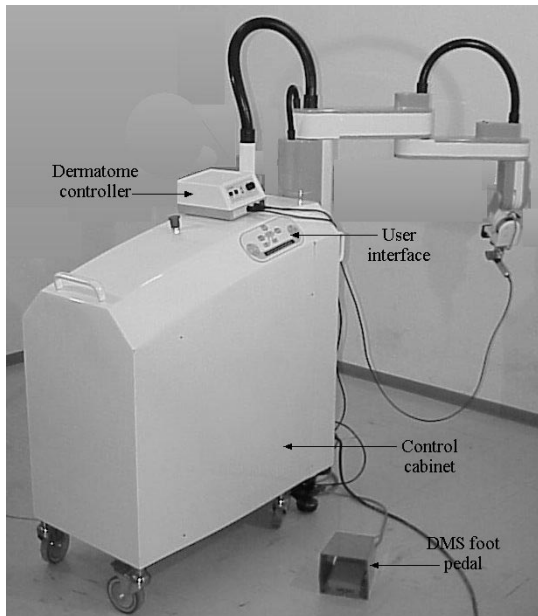
Fig. 5. DERMAROB arm and the control cabinet.
