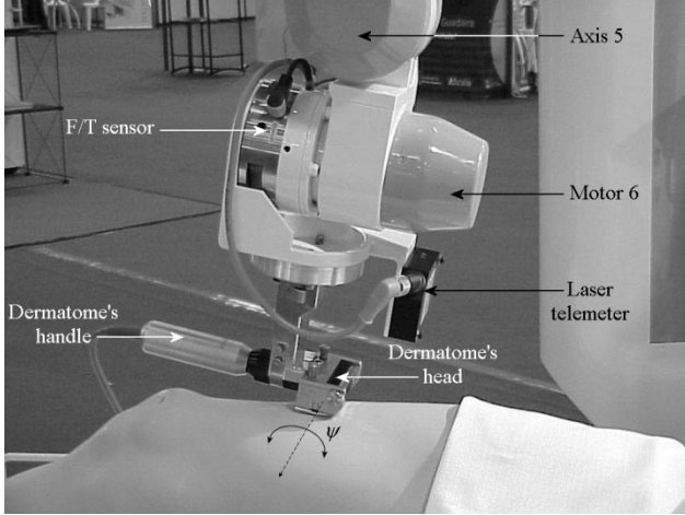
Fig. 7. Close-up of the Dermarob wrist.
