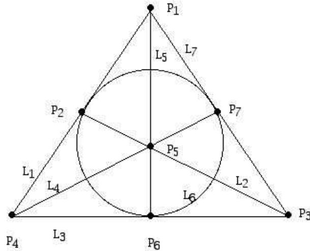
Figure 1. The Fano plane
