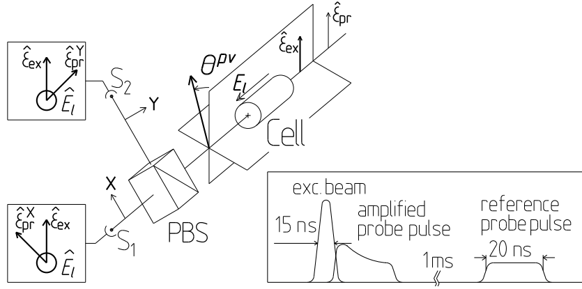
Fig. 2. Schematic of the ENS-Paris pump-probe Cs experiment showing the two orthogonal symmetry planes defined by the electric field \mathbf{E} and the linear excitation polarization \hat{\epsilon}_{ex} . APV gives rise to a tilt \theta^{pv} of the optical axes of the excited vapor out of those planes. The incoming probe polarization \hat{\epsilon}_{pr} provides a superposition of the right- and left-handed ( \hat{\epsilon}_{ex}, \hat{\epsilon}_{pr}, \mathbf{E} ) configurations analyzed. The probe amplification difference is directly extracted from the optical signals S_1, S_2 , recorded in each channel of the Polarizing Beam Splitter (PBS). Inset: timing of the experiment repeated at \sim 150 Hz. (Fig. adapted from Guéna et al. 39 ).
