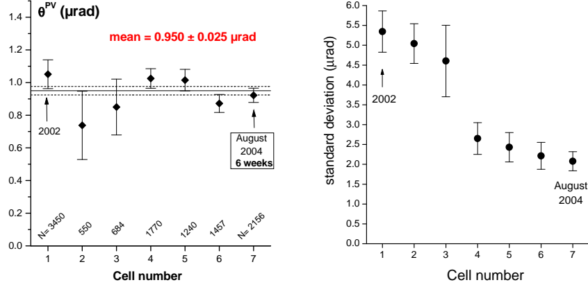
Fig. 3. Results of the ENS experiment. Left: Values of \theta^{PV} = -Im E_1^{pv} / \beta E obtained in different Cs cells: mean (diamond) and statistical error (error bar) from the sample of N data acquired in each of the 7 cells. Solid and dashed lines: global mean and statistical error, respectively. Right: Standard deviation of the distribution of the PV data relative to each cell. Adapted from Ref. 43 .
