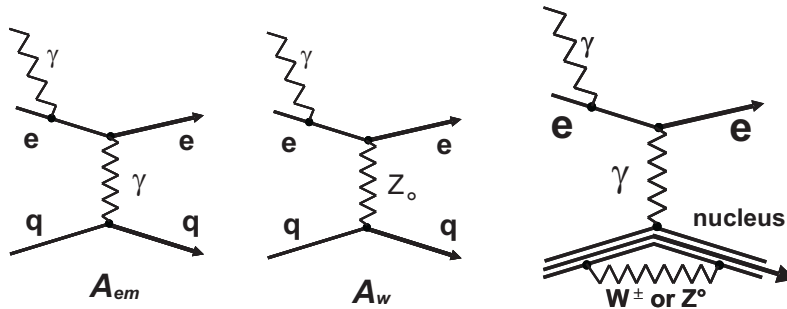
Fig. 1. Left and center: Schematic representation of the two amplitudes, electromagnetic A_{em} and weak A_W associated with a photon or Z_0 exchange between electron e and quark q , which can contribute to the same radiative process and give rise to an electroweak interference. Right: Schematic representation of the nuclear-spin-dependent PV interaction associated with the nuclear anapole moment.
