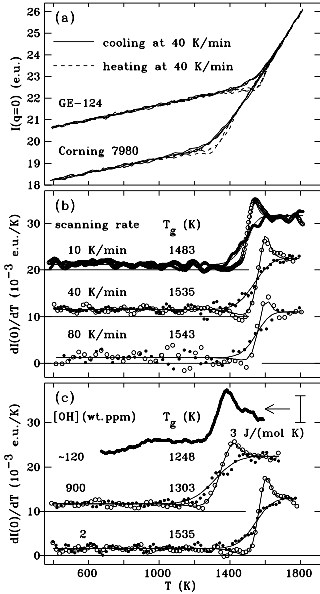
Fig. 2 – (a) Scattered intensity, extrapolated to q = 0 , as a function of temperature. GE-124 contains 2 wt. ppm \text{H}_2\text{O} , and Corning 7980 contains 900 wt. ppm \text{H}_2\text{O} . (b) Temperature derivatives of I(0) , obtained for GE-124 upon scanning the temperature at different rates. Full and open symbols show cooling and heating data, respectively. Solid lines are fits to the AGF equation. For clarity, the 40 and 10 K/min curves were shifted up by 10 and 20 \times 10^{-3} e.u./K, respectively. (c) Temperature derivatives of I(0) data obtained at 40 K/min for GE-124 and, shifted up by 10 \times 10^{-3} e.u./K, Corning 7980. Top: heat flow upon heating a sample with \approx 120 wt. ppm at 40 K/min (ref. [3]).
