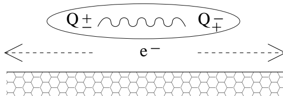
FIG. 2: Schematic description of entangled quasiparticles Q_\pm being emitted right and left of the tunnel junction.
