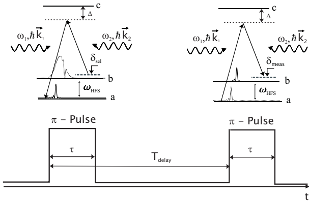
Fig. 2. Principle of the velocity sensor, the first \pi -pulse transfers a narrow velocity class from the level |b\rangle to the level |a\rangle (selection) and the second \pi -pulse transfers the accelerated atoms back to the level |b\rangle (measurement).
