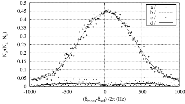
Fig. 4. a) Final velocity distribution of atoms in hyperfine state |F = 2, m_F = 0\rangle measured using two counter-propagating Raman beams and normalized to N_{\text{sel}} = N_a + N_b the number of atoms selected by the first pulse ( N_a and N_b are successively the number of atoms measured in the hyperfine states |F = 1, m_F = 0\rangle and |F = 2, m_F = 0\rangle ). b) Theoretical fit. c) Difference between the experimental data and the theoretical fit. d) Smoothing curve of the last data using a fixed window. We note finally that in x-axis the velocity is expressed in terms of frequency.
