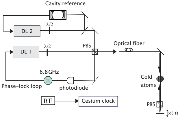
Fig. 3. Experimental setup of the velocity sensor: The two laser diodes are phase locked using a tunable microwave chain. The two Raman beams with \text{lin}\perp\text{lin} polarizations are injected into the same optical fiber. After passing through the vacuum chamber only the beam k_2 is retroreflected by the horizontal mirror allowing a counter-propagating excitation.
