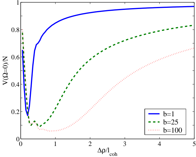
FIG. 6: Squeezing spectrum at zero-frequency, normalized to the shot noise, as a function of the radial amplitude of the detector scaled to l_{coh} , plotted for several values of b
