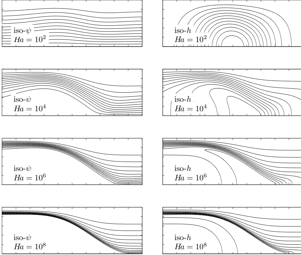
FIGURE 9. FreeFem calculations: velocity and electric current streamlines, iso- \psi and iso- h on the left and right respectively for 4 values of the Hartmann number, Ha = 10^2, 10^4, 10^6, 10^8 . The vertical coordinate is the y coordinate from y = 0 (centerline of the duct) to y = 0.5 , the horizontal coordinate is x from x = -2 to x = 2 .
