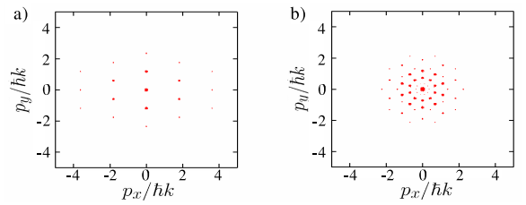
FIG. 2: Matterwave interference pattern of a BEC released from a combined OL and harmonic trap: a) periodic case; b) quasi-periodic case. Both correspond to ^{87}\text{Rb} and V_0 = -10E_R , where E_R = \hbar^2 k^2 / 2M is the recoil energy.
