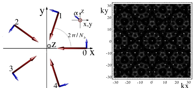
FIG. 1: Left: laser arrangement (see text for details). Right: Quasi-periodic lattice potential for N_b = 5 , V_0 < 0 and \alpha_j = 0 . White points correspond to potential minima.
