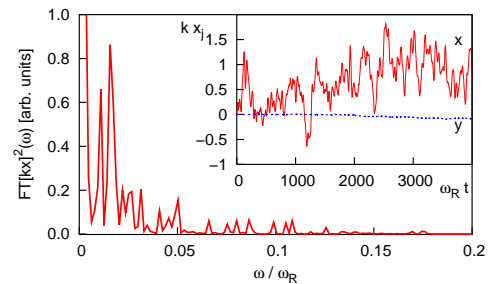
FIG. 4: Fourier transform of the mean position of a BEC in a periodic or quasiperiodic lattice. Inset: Time evolution of a BEC in a tilted quasiperiodic lattice. All beams have the same intensity, V_0 = -2E_R and V_{\text{tilt}} = 0.002E_R \times kx .
