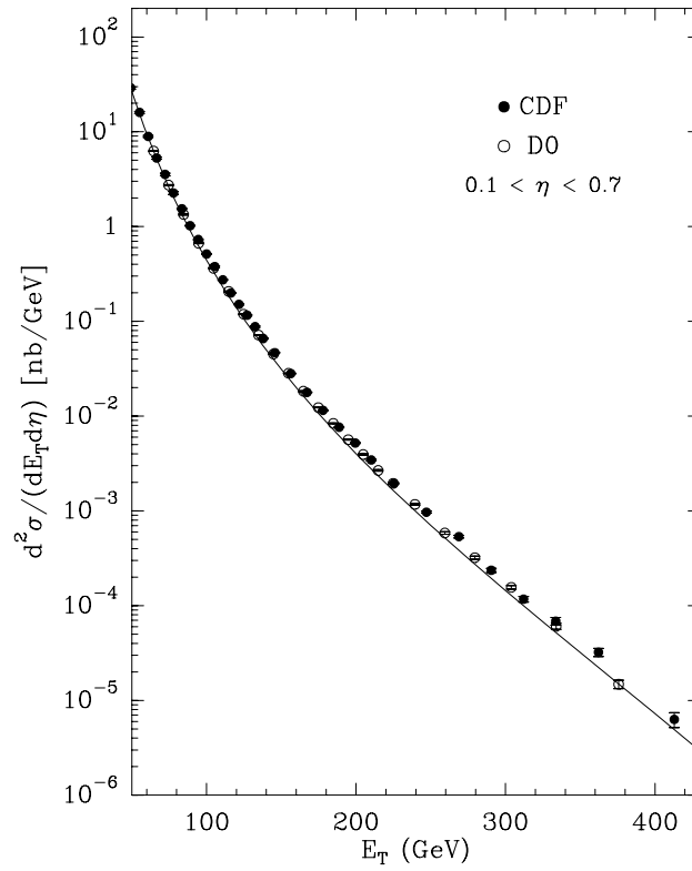
Figure 19: Cross section for single jet production in \bar{p}p at \sqrt{s} = 1.8\text{TeV} as a function of E_T . Data are from CDF [36] and D0 [37] experiments.
