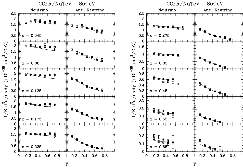
Figure 15: Differential cross section \nu(\bar{\nu})N for E_\nu = 85\text{GeV} , as a function of y . Data are from CCFR [29] (white circles) and NuTeV experiments [30, 31] (black circles).
