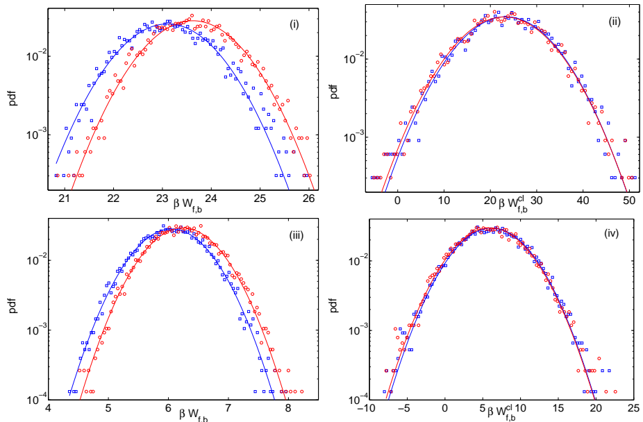
Figure 3: Case a): (i) P_f(W) and P_b(-W) , (ii) P_f(W^{cl}) and P_b(-W^{cl}) ; Case c): (iii) P_f(W) and P_b(-W) , (iv) P_f(W^{cl}) and P_b(-W^{cl}) (experimental forward and backward pdfs are represented by \circ and \square respectively, whereas the continuous lines are Gaussian fits)
