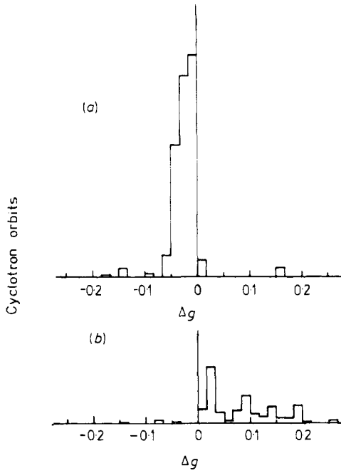
Figure 11. Histograms of the mean \Delta g values over cyclotron orbits, for (a) the second and (b) the third zone. The distribution tails of figures 7 and 8 are absent here.
