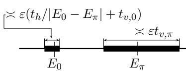
(a) When |E_\pi - E_0| \gg \varepsilon t_{v,\pi}(\bar{E})
