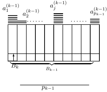
Figure 1: k^{th} -tower.
