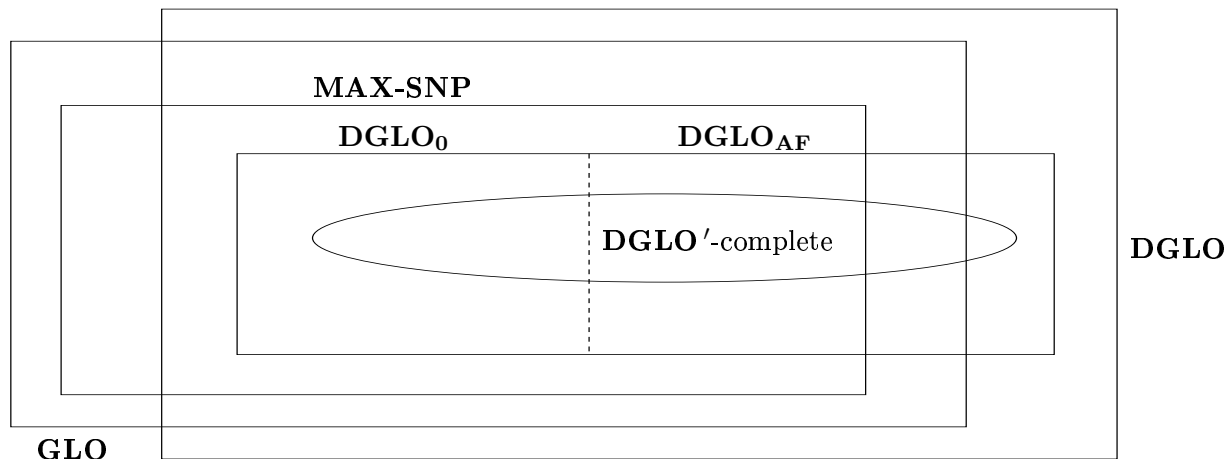
Figure 3: \mathbf{GLO} , \mathbf{DGLO} , \mathbf{MAX-SNP} , \mathbf{DGLO}' = \mathbf{DGLO}_0 \cup \mathbf{DGLO}_{\mathbf{AF}} , \mathbf{DGLO}' -complete.
