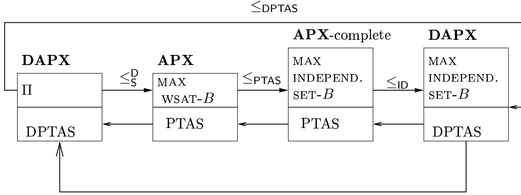
Figure 2: The schema of the proof of Theorem 4.
