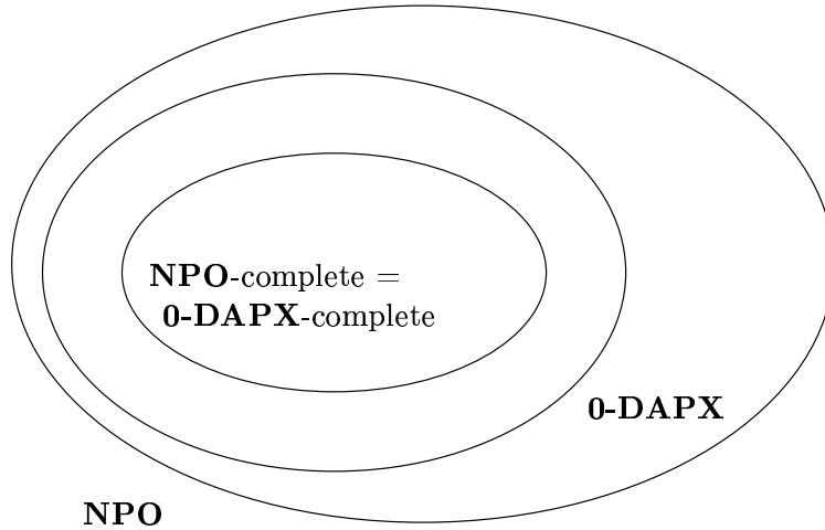
Figure 1: Class inclusions and completeness under D reduction.
