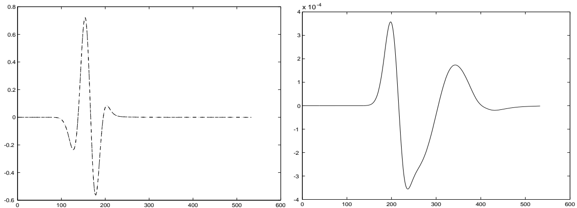
Figure 4: Pressure field (left) and error on the pressure (right) near the upperleft corner for a horizontal flow M = 0.33 vs. time steps
