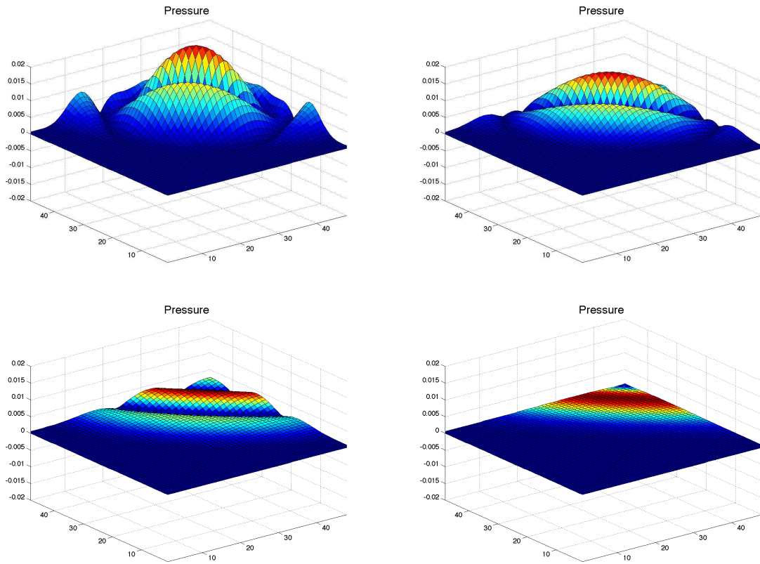
Figure 2: Pressure field for an oblique velocity M = 0.9 at successive time steps
