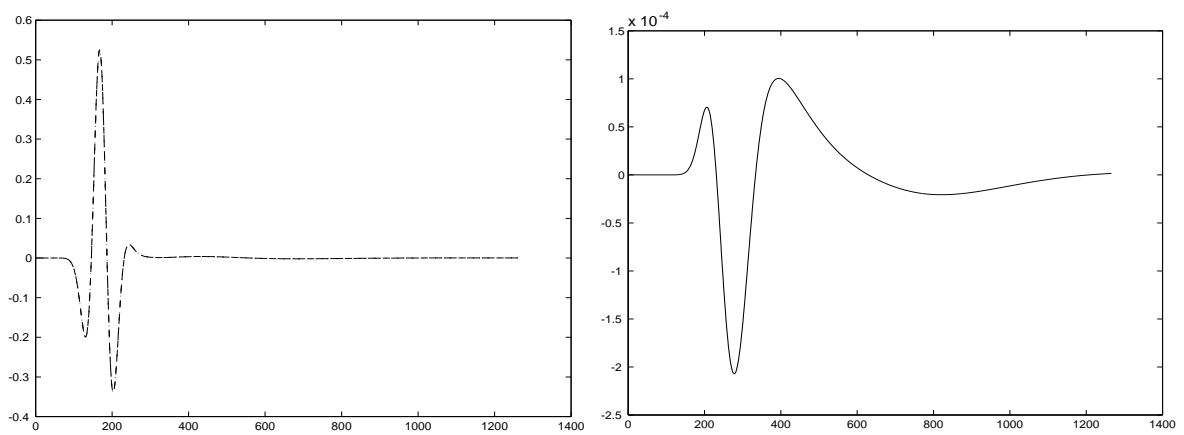
Figure 3: Pressure field (left) and error on the pressure (right) near the upperleft corner for an oblique velocity M = 0.9 vs. time steps
