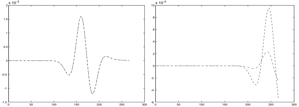
Figure 1: Pressure fields for the reference solution and the PML solution near the upperleft corner (left) and in the PML (right) for an oblique flow M = 0.33 vs. time steps
