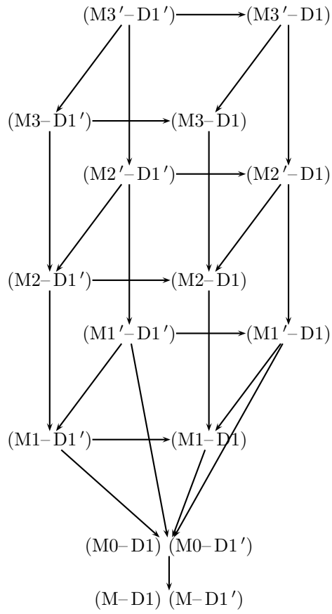
Figure 1: Graph of implications
