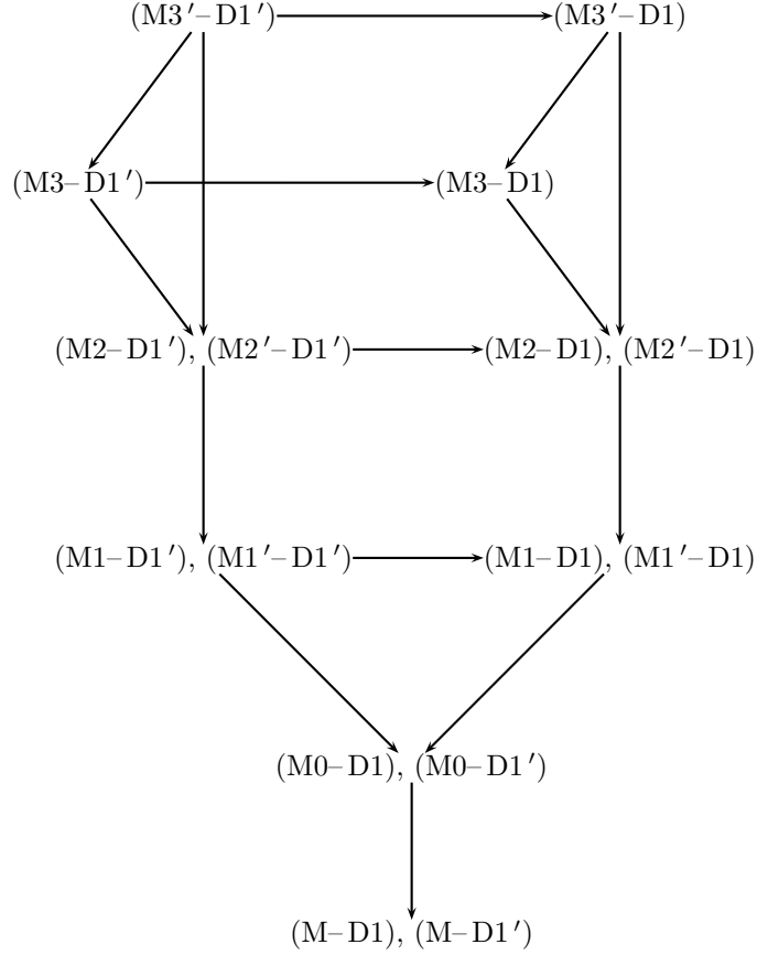
Figure 2: Distinct models and implications in the non-denumerable case
