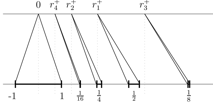
Figure 3: Transformation of \varphi into \psi
