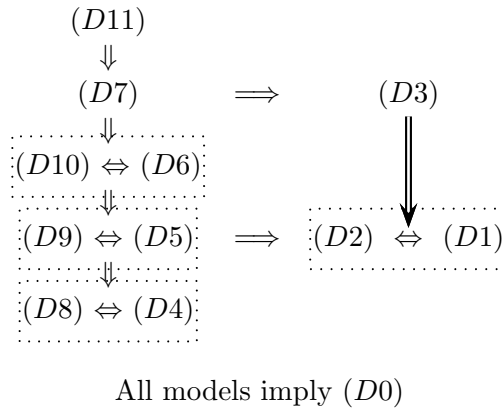
Figure 4: Implication between models resulting from theorem 5.1
