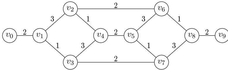
Figure 5: Gadget F_2 for e \in E_2 .
