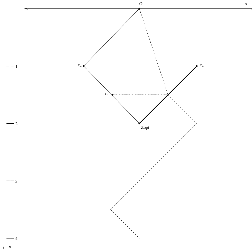
Fig. 1. A graphical example of the lower bound for general metric spaces. The plain line on the left is the tour of the optimal server, while the dashed line is the tour of the on-line server. As soon as the on-line server crosses the (virtual) bold line, a new request is released in the symmetric point (with respect to the origin). Any on-line tour that serves two requests can not end before time 4, while Z^* = 2
