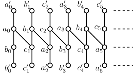
FIGURE 5. A pattern in T .
