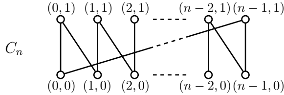
FIGURE 3. The crown C_n .
