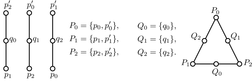
FIGURE 1. The poset P and the geometry of \mathbf{K} .
