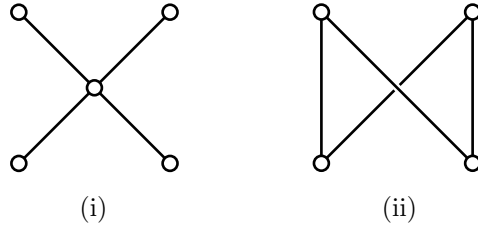
FIGURE 4. A tree-like poset which contains the crown C_2 .
