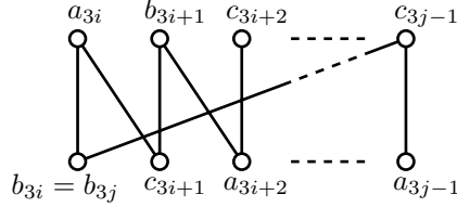
FIGURE 7. A pre-crown in T .
