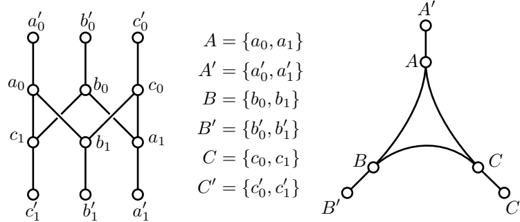
FIGURE 2. The poset Q and the geometry of \mathbf{L} .
