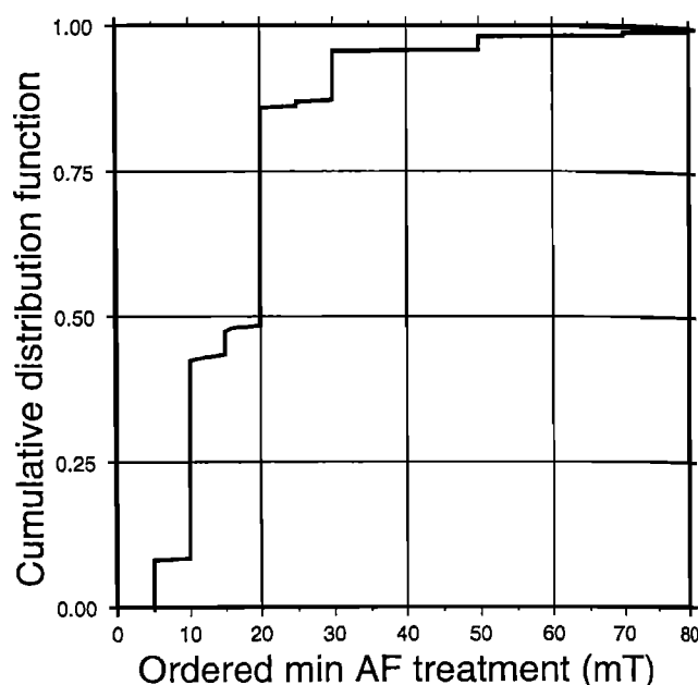
Figure 5. Cumulative distribution function of the first AF value used in the least squares analysis to compute the direction of ChRM.
