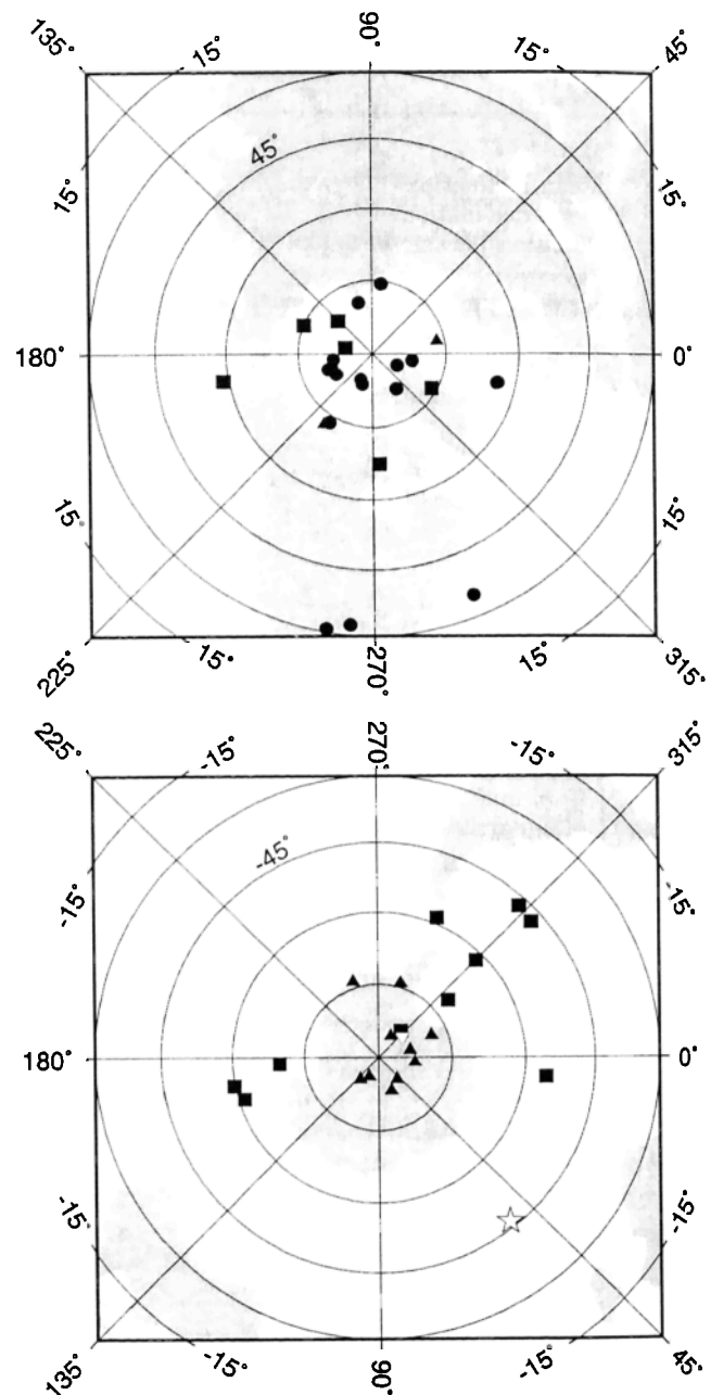
Figure 7. Virtual geomagnetic pole positions for Possession Island lava flows. Equal Area projection of a portion of (a) Northern and (b) Southern Hemisphere. Circles, AL section; solid triangles, PC section; open triangles, BO unit; squares, CN section.
