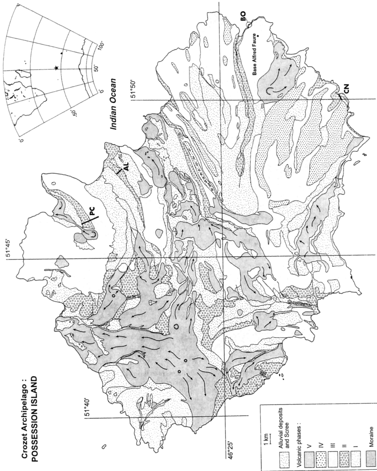
Figure 1. Sketch showing locations of sampled sections on a geological map redrawn from Chevallier [1981].
