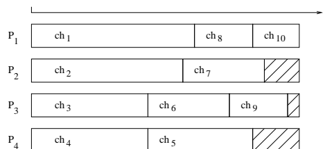
Figure 9: LPT principle of allocation on four processors.
