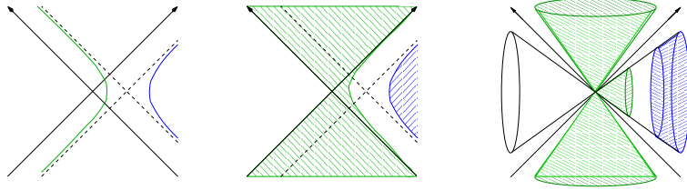
Figure 1.2 Closed string worldsheets in Misner space are obtained by smearing the trajectory of a charged particle in Minkowski space with a constant electric field. Short (resp. long) strings correspond to charged particles which do (resp. do not) cross the horizon.
