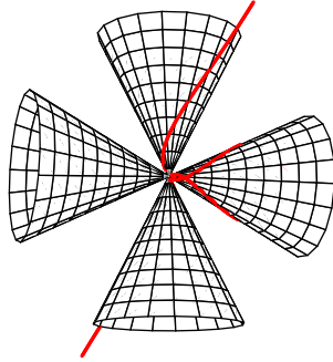
Figure 1.1 Free particles or untwisted strings propagate from the past Milne region to the future Milne region, with a temporary excursion in the whiskers.
