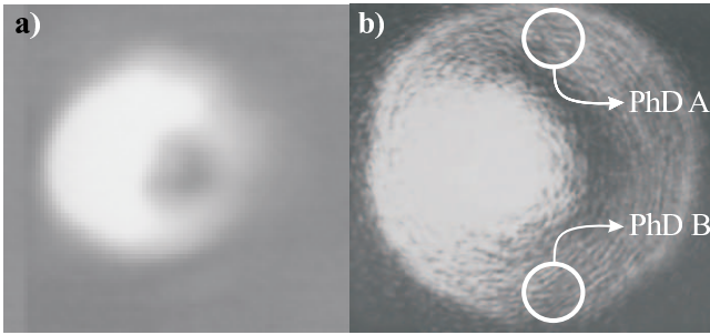
FIG. 2: Image of the non linear emission in RS (a) and in \mathbf{k} -space (b) in the degenerate geometry [16]. Cavity exciton detuning 0.3 meV and laser intensity 2.2 mW. In (a) the dark region in the laser spot corresponds to the polariton resonance. In (b) the polariton emission is seen around the (brighter) reflected laser in \mathbf{k} -space, showing a larger angular divergence. The principle of the intensity correlation measurement is schematically indicated.
